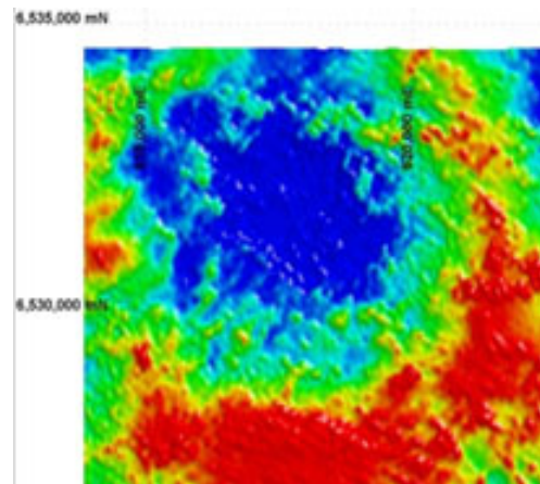
Apollo Topography
